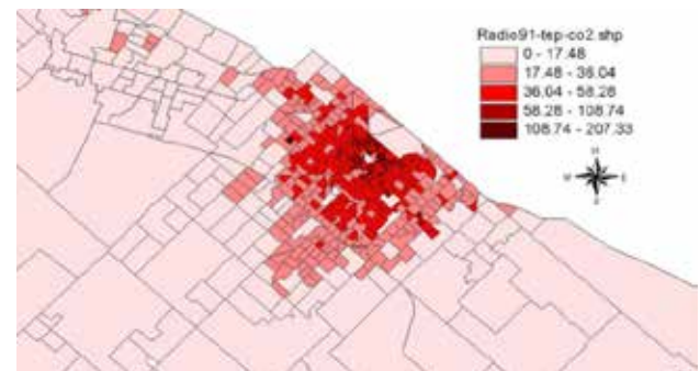
Figure 12. Total energy density of the Residential sector per census radio. TEPC/Hectare.year
